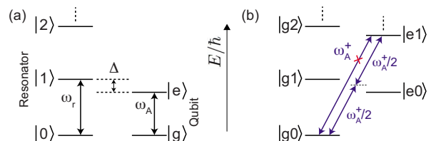
FIG. 1. (Color online) (a) Schematic of the energy levels of a harmonic oscillator with resonant frequency \omega_r , and levels |n\rangle corresponding to photon number n and qubit with transition frequency \omega_A and ground and first-excited states |g\rangle and |e\rangle , respectively. (b) Combined level diagram, indicating the blue sideband transition \omega_A^+ = \omega_r + \omega_A , which with one photon is forbidden to first order, but may be driven using two photons, for example, both at a frequency of \omega_A^+/2 .
